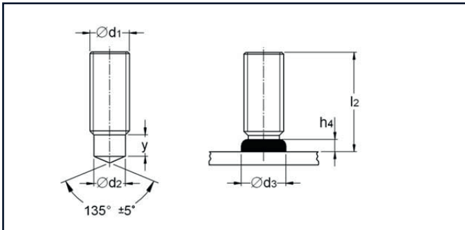
Threaded stud PD, dimensions acc. to EN ISO 13918
